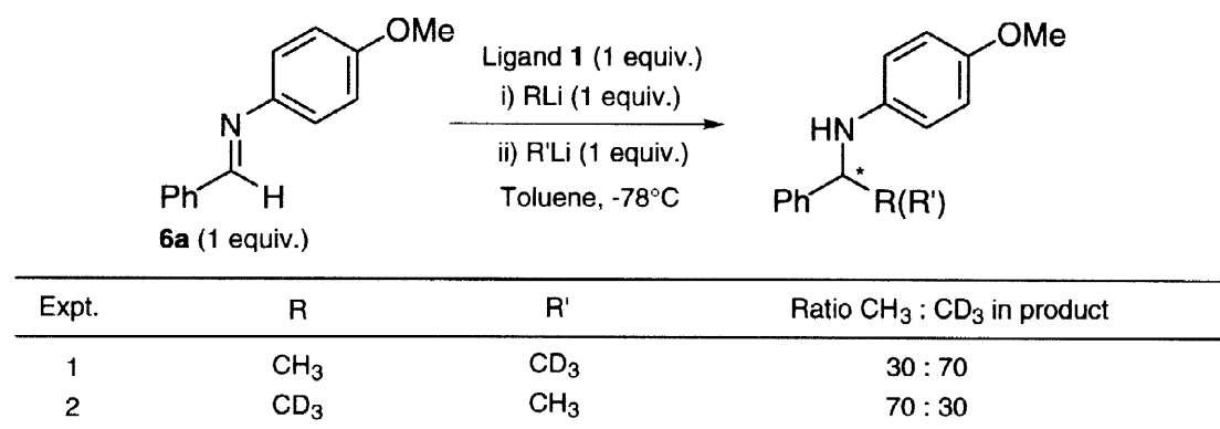
Scheme 2. Deuterium-labelling studies of the addition of methyllithium to 6a mediated by ligand 1 .
